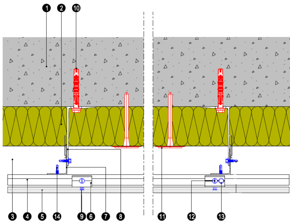
Figure 17– Coupe horizontale
