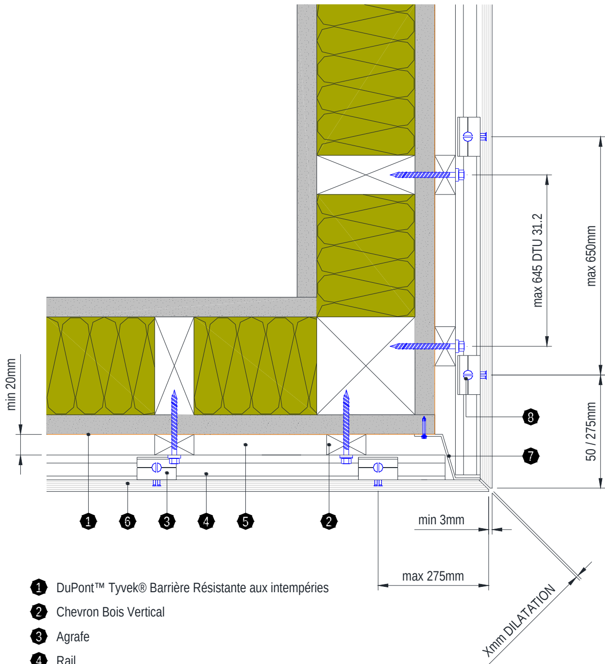
Figure 41.5 - Angle biseauté
