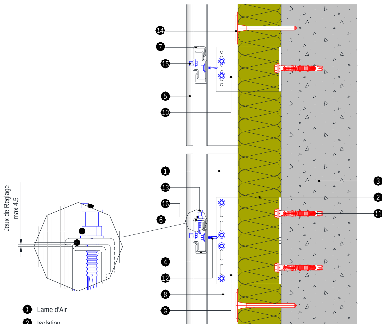
Figure 16 – Coupe verticale
